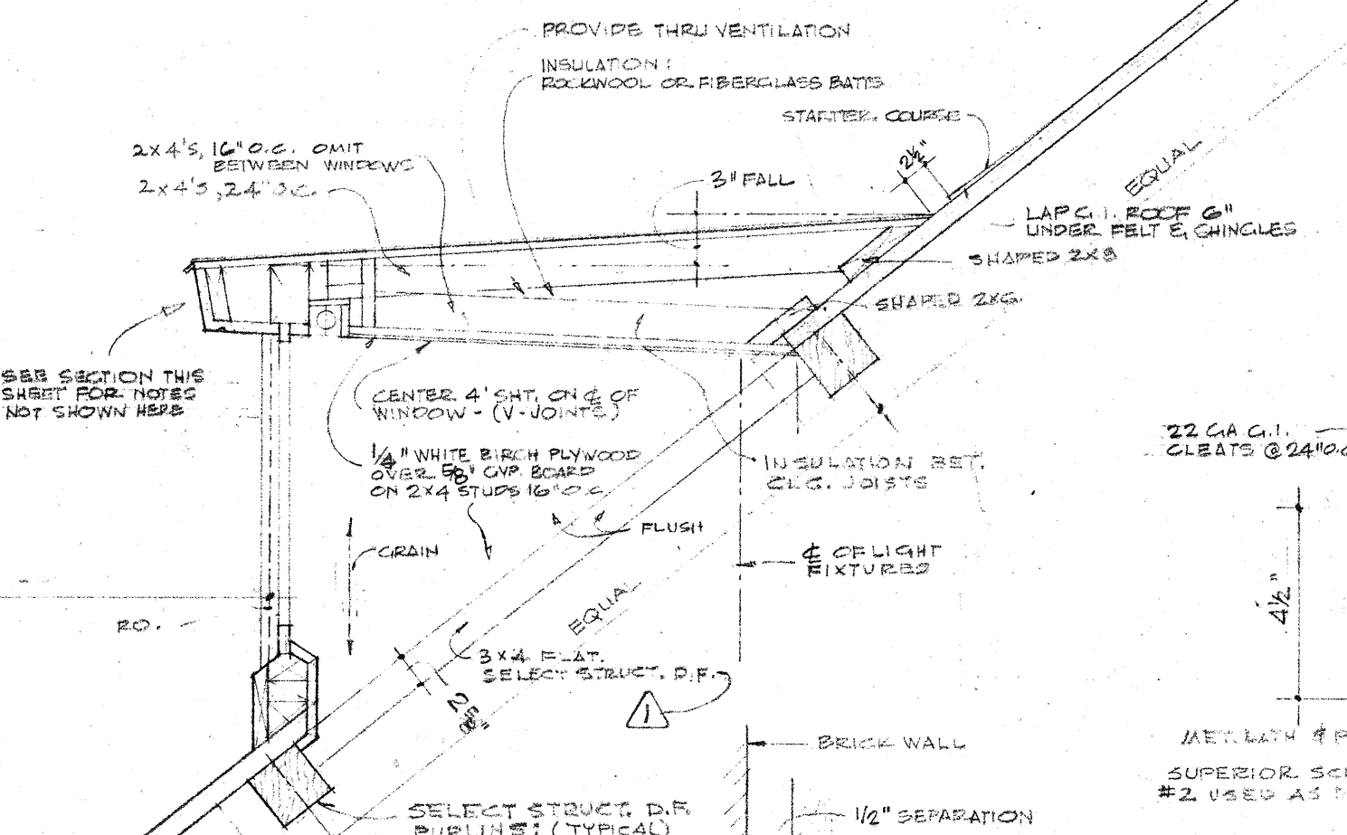
TYPICAL END ELEVATION OF DORMER SCALE 3/4" = 1'-0"
