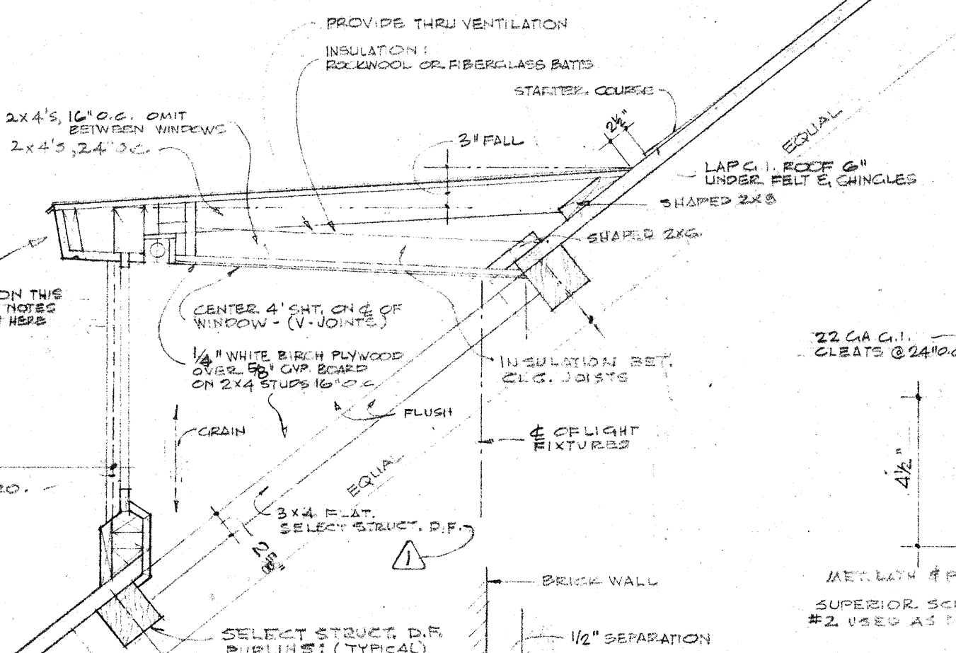
TYPICAL END ELEVATION OF DORMER SCALE 3/4" = 1'-0"
