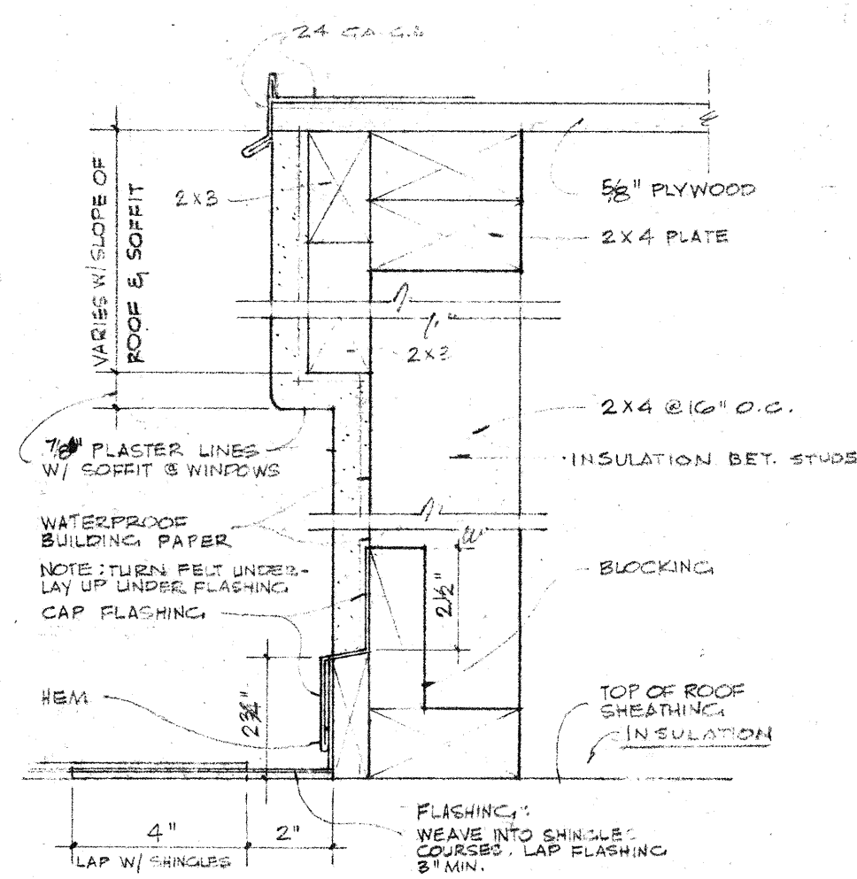
A SECTION THRU ENDS OF DORMERS SCALE 3/4" = 1'-0"
